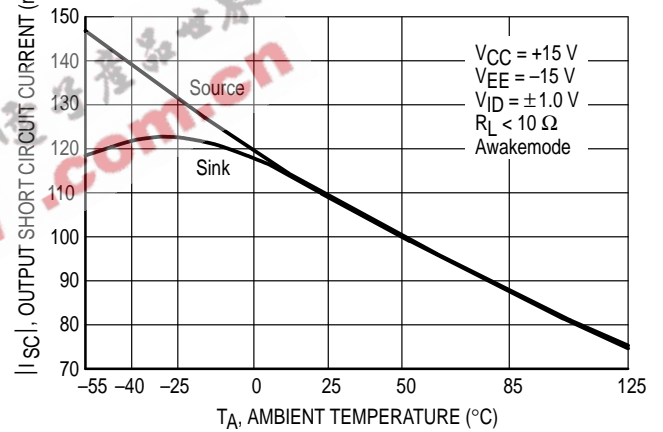
Figure 16. Output Short Circuit Current versus Temperature
