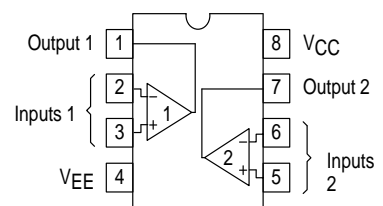
(Dual, Top View)
