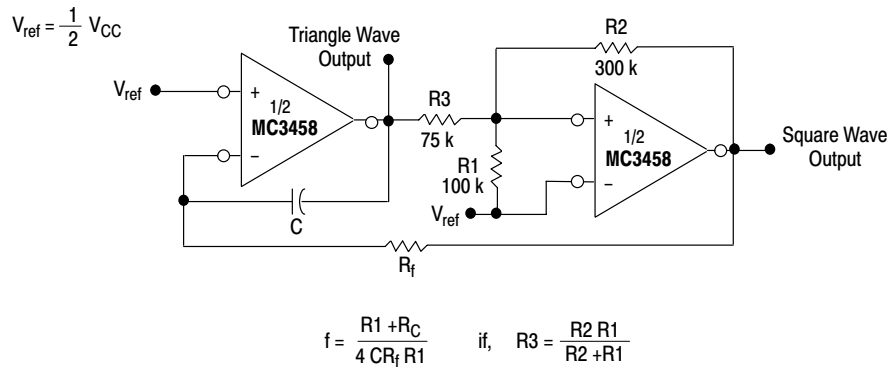
Figure 14. Function Generator
