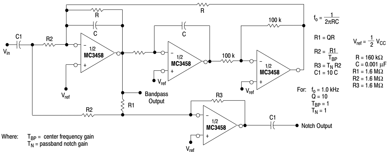
Figure 13. Bi-Quad Filter
