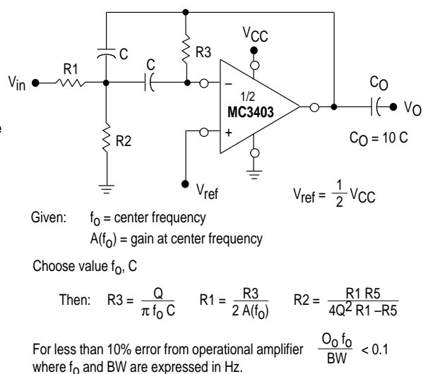
Figure 13. Multiple Feedback Bandpass Filter
