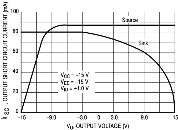
Figure 14. Output Short Circuit Current versus Output Voltage
