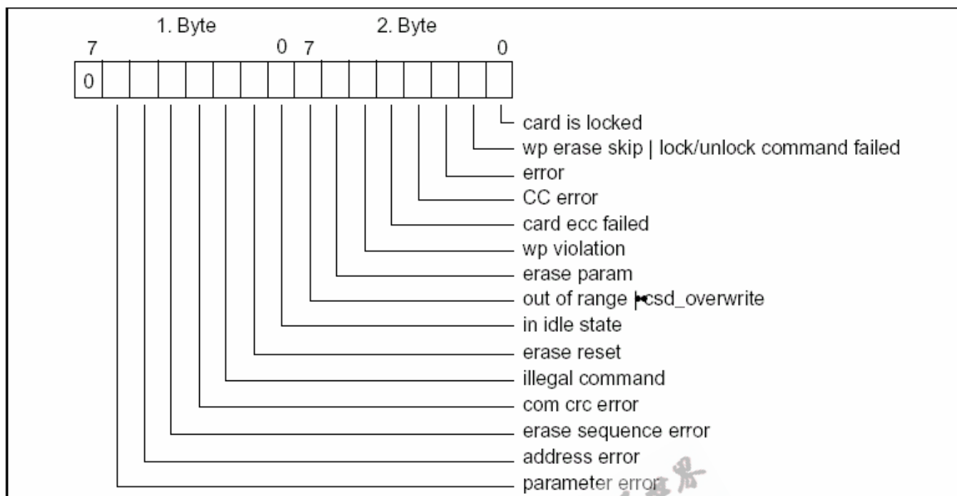
Figure 4-10 R2 Response Format
