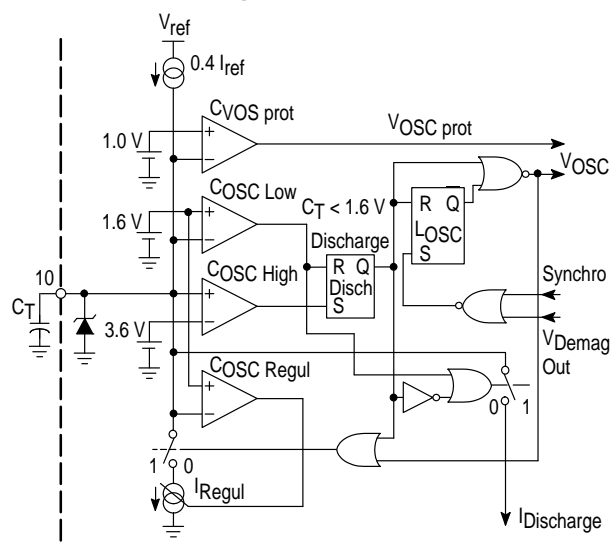
Figure 34. Oscillator
