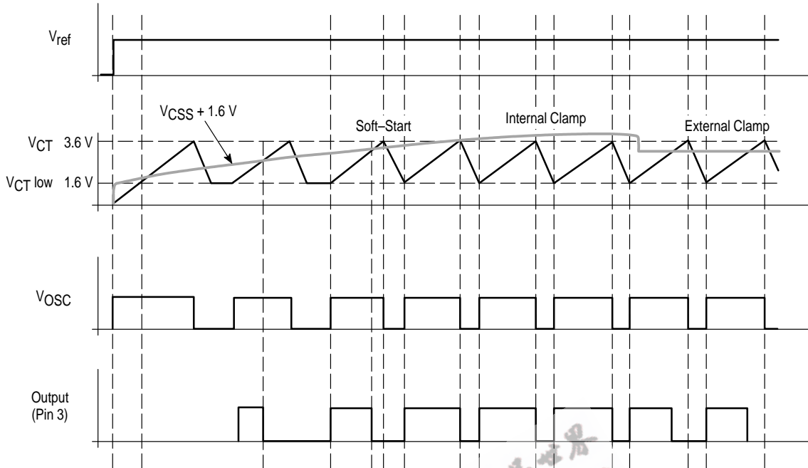
Figure 31. Soft-Start & Dmax
