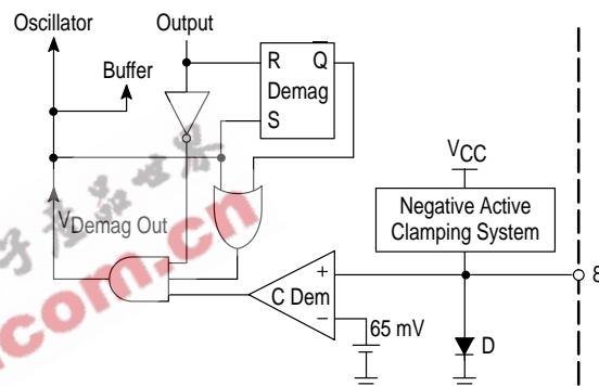
Figure 38. Demagnetization Block
