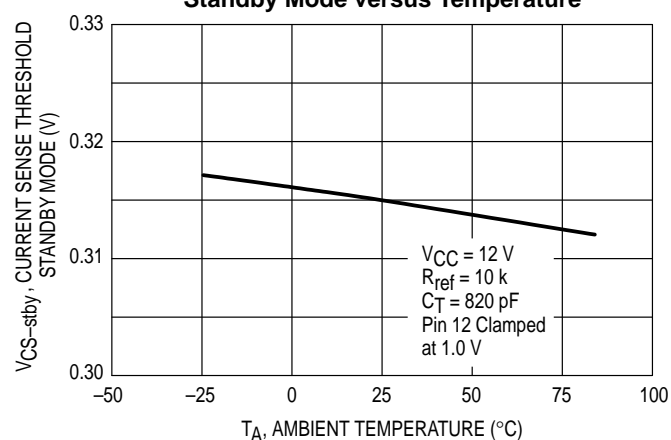
Figure 26. Current Sense Voltage Threshold Standby Mode versus Temperature
