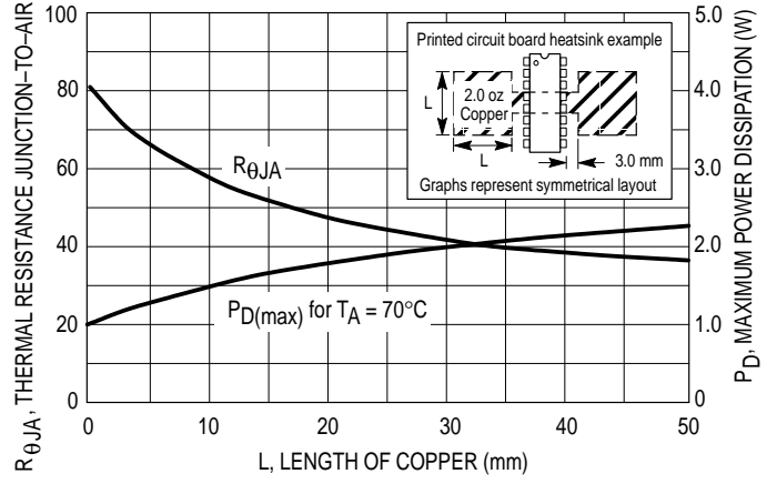
Figure 14. Thermal Resistance and Maximum Power Dissipation versus P.C.B. Copper Length
