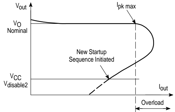
Figure 45. Foldback Characteristic
