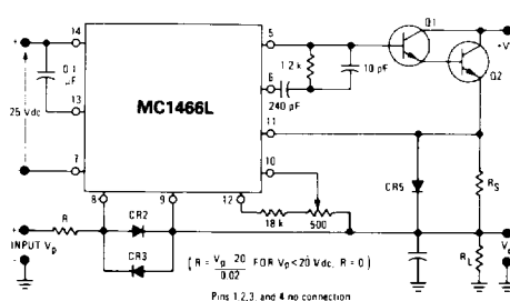
FIGURE 4 — REMOTE PROGRAMMING
