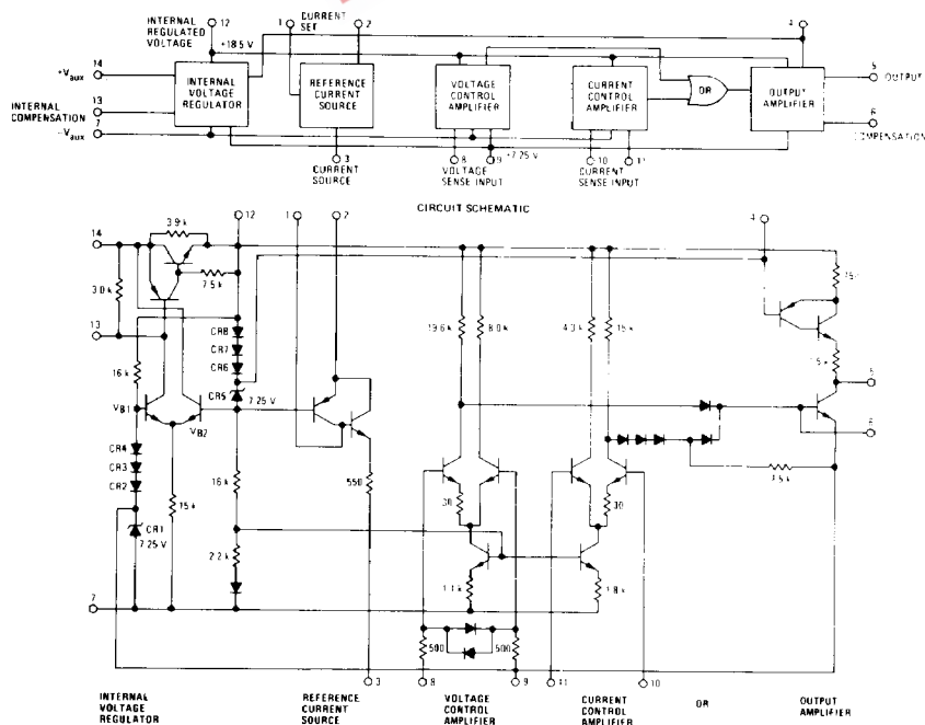
FIGURE 5 — BLOCK DIAGRAM
