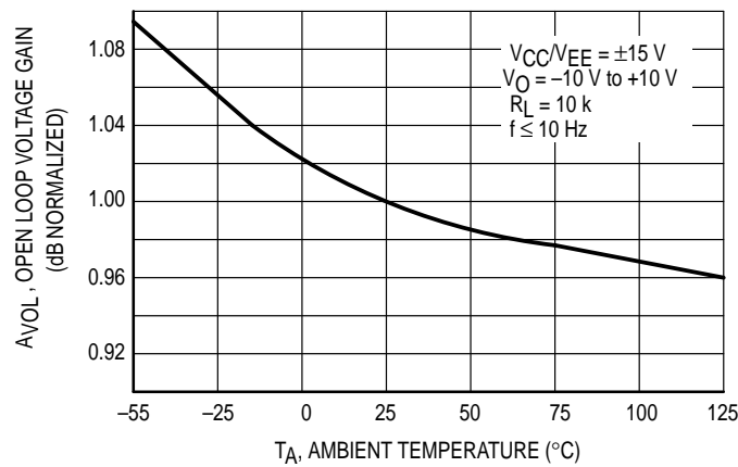
Figure 13. Open Loop Voltage Gain versus Temperature
