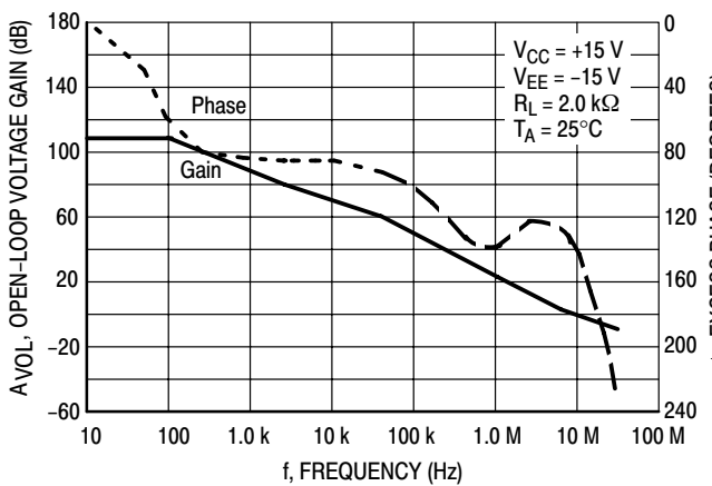
Figure 26. Voltage Gain and Phase versus Frequency
