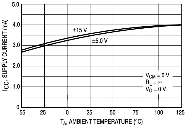
Figure 10. Supply Current versus Temperature
