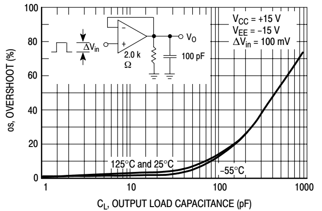
Figure 29. Overshoot versus Output Load Capacitance
