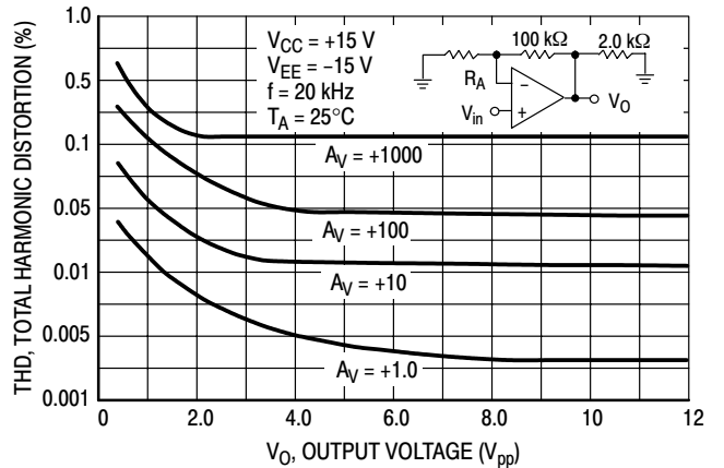
Figure 23. Total Harmonic Distortion versus Output Voltage
