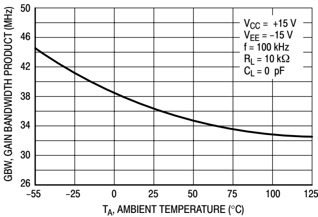
Figure 14. Gain Bandwidth Product versus Temperature
