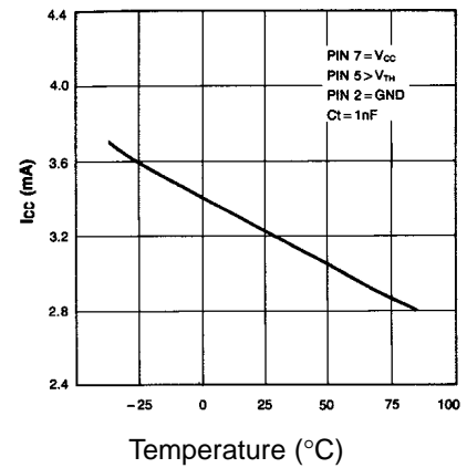
Figure 2. Temperature Drift ( I_{CC} )
