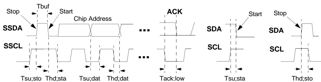
Figure 10. SSDA/SSCL Timing
