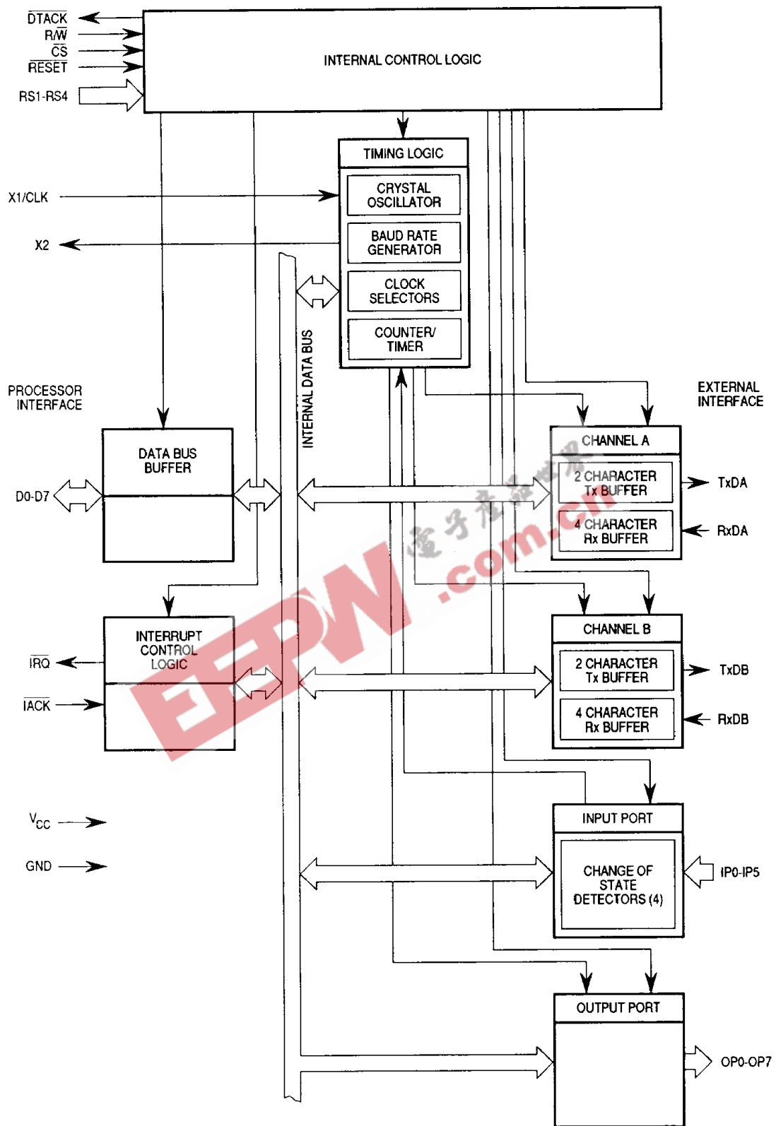
Figure 1. Block Diagram
