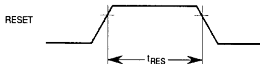
Figure 3. RESET Timing
