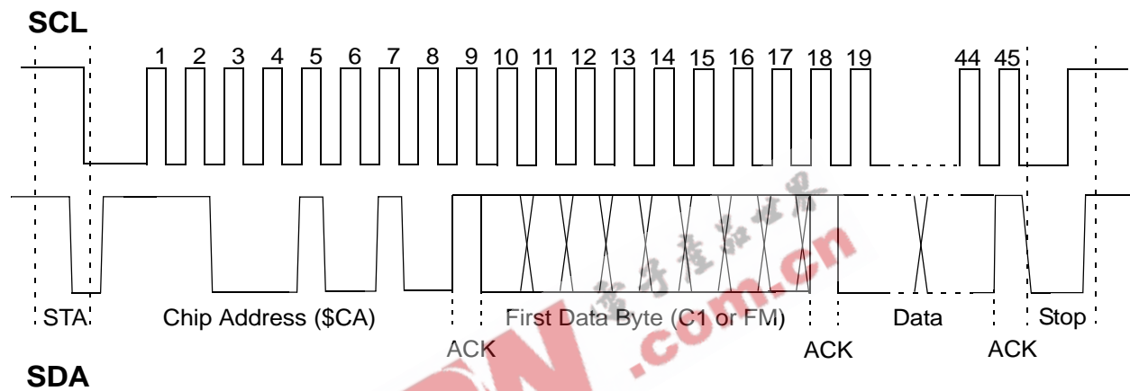
Figure 12. I 2 C Bus Timing
