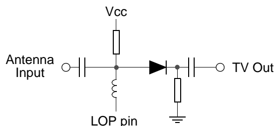
Figure 7. Typical Attenuator Application with Pin Diode
