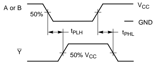
Figure 4. Switching Waveforms
