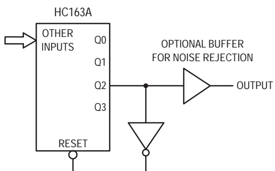
Figure 13. Modulo-5 Counter
