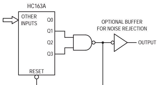
Figure 14. Modulo-11 Counter
