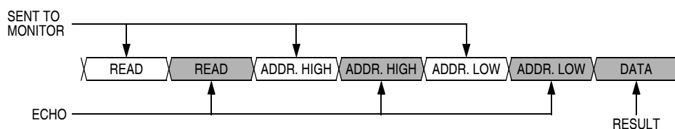
Figure 9-4. Read Transaction
