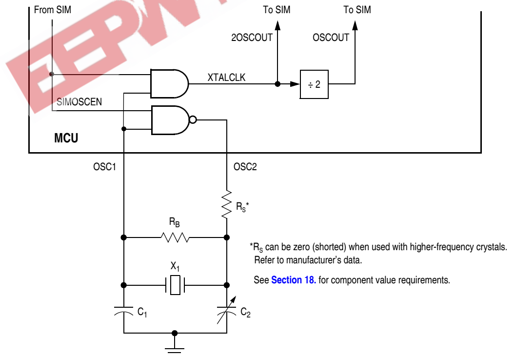
Figure 8-1. X-tal Oscillator External Connections
