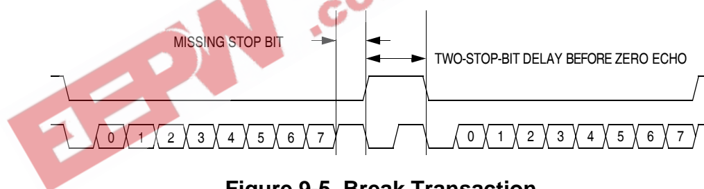
Figure 9-5. Break Transaction
