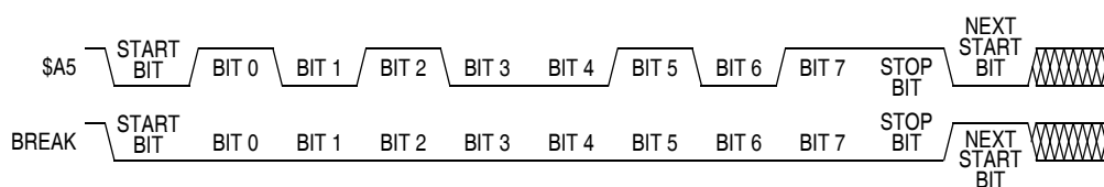
Figure 9-3. Sample Monitor Waveforms
