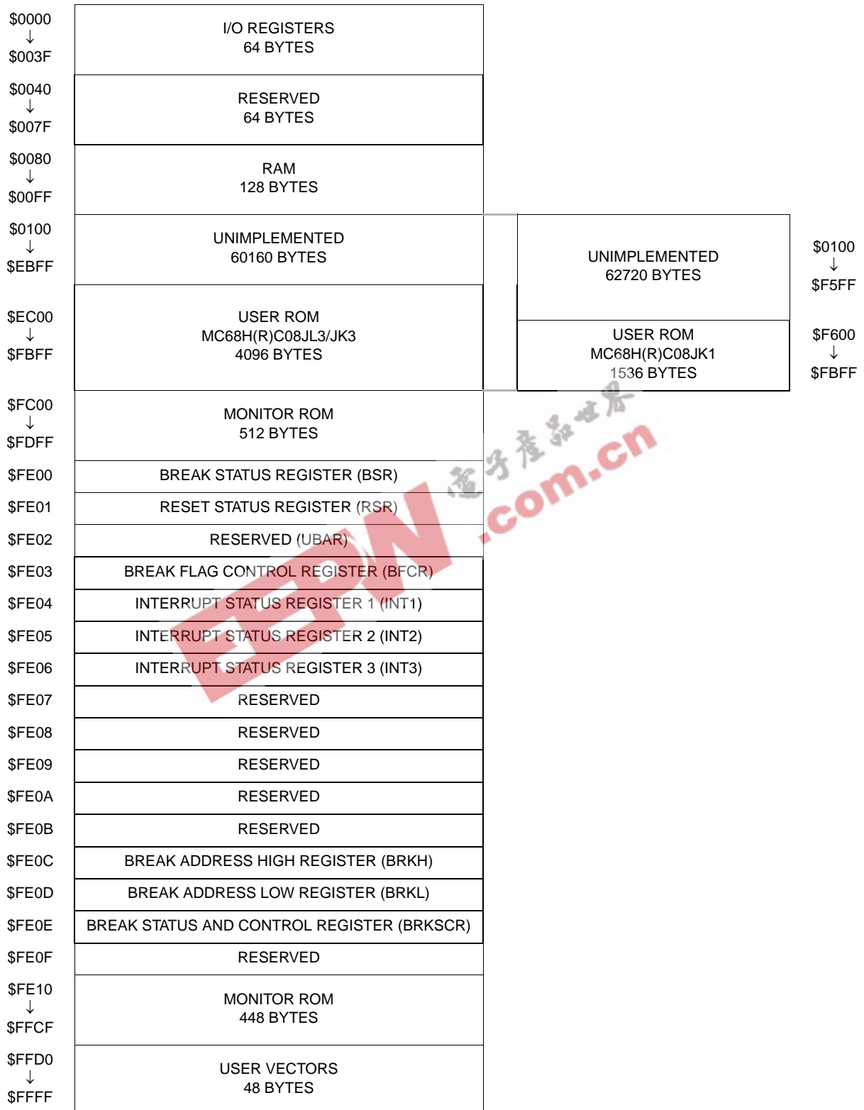
Figure 2-1. Memory Map
