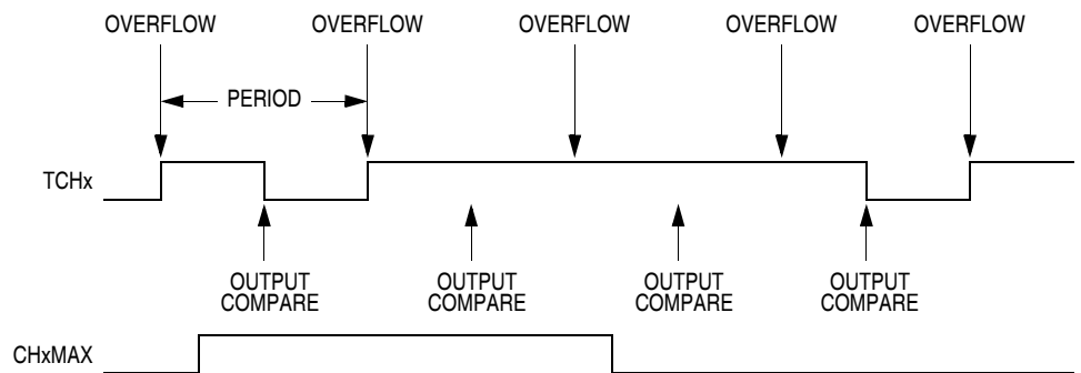
Figure 10-8. CHxMAX Latency
