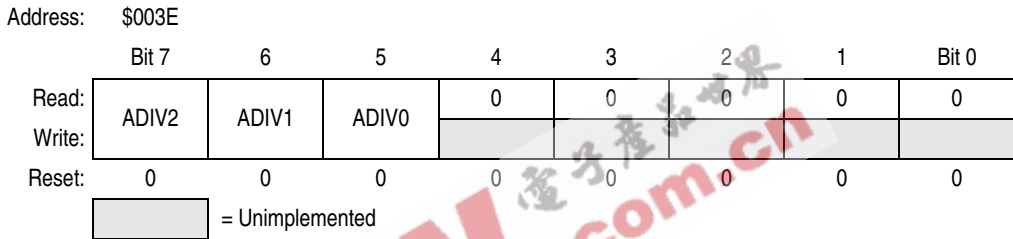
Figure 9-5. ADC Input Clock Register (ADICK)
