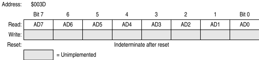
Figure 9-4. ADC Data Register (ADR)
