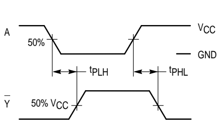
Figure 1. Switching Waveforms
