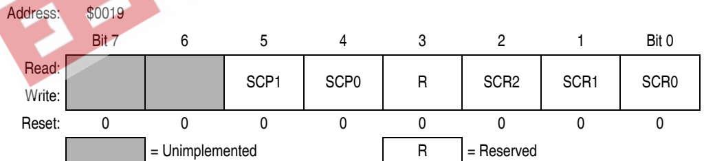
Figure 13-17. SCI Baud Rate Register (SCBR)
