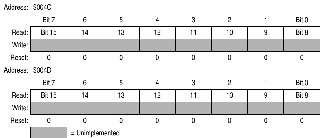
Figure 11-4. PIT Counter Registers (PCNTH–PCNTL)
