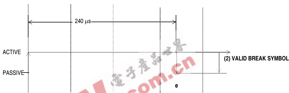
Figure 4-12. J1850 VPW Received BREAK Symbol Times
