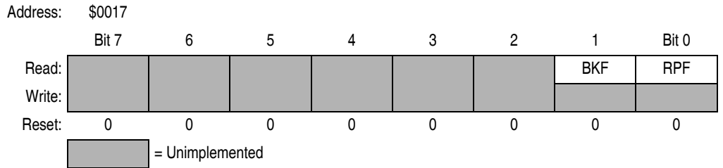
Figure 13-15. SCI Status Register 2 (SCS2)
