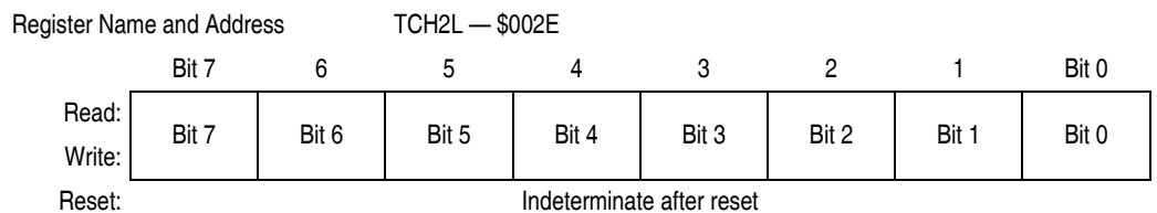
Figure 16-10. TIM Channel Registers (TCH0H/L–TCH3H/L)
