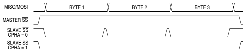
Figure 15-13. CPHA/SS Timing
