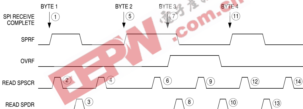
Figure 15-9. Missed Read of Overflow Condition
