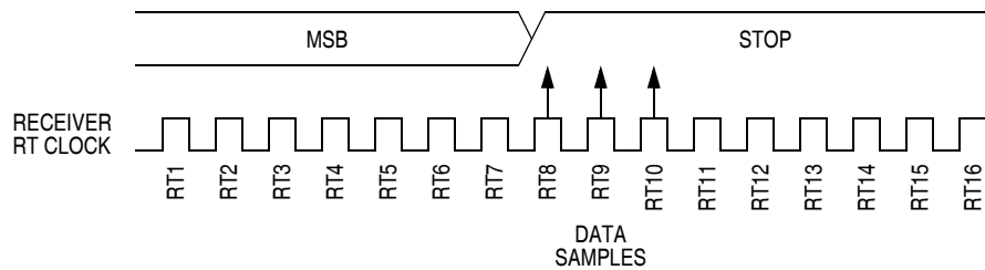
Figure 13-8. Slow Data
