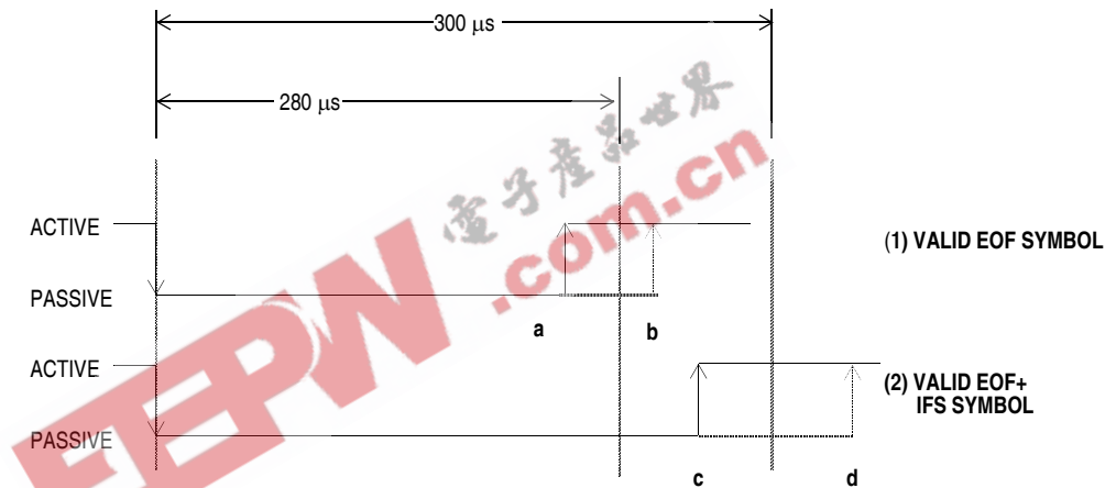
Figure 4-10. J1850 VPW Received Passive EOF and IFS Symbol Times
