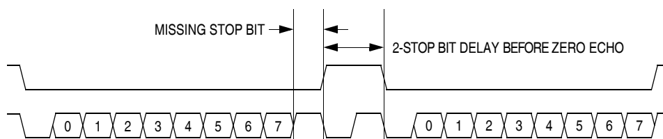
Figure 17-9. Break Transaction
