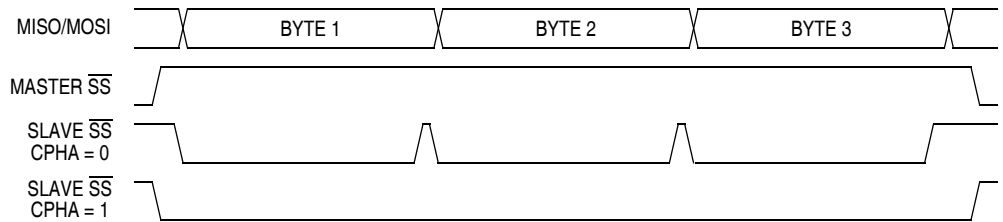
Figure 15-6. CPHA/ \overline{SS} Timing
