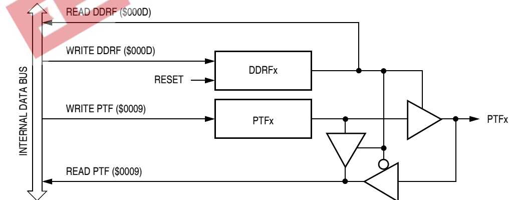
Figure 12-19. Port F I/O Circuit
