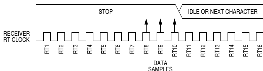
Figure 13-9. Fast Data
