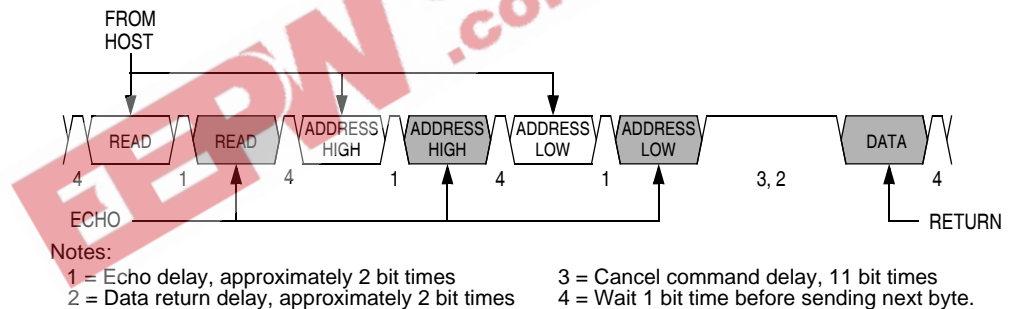
Figure 17-10. Read Transaction
