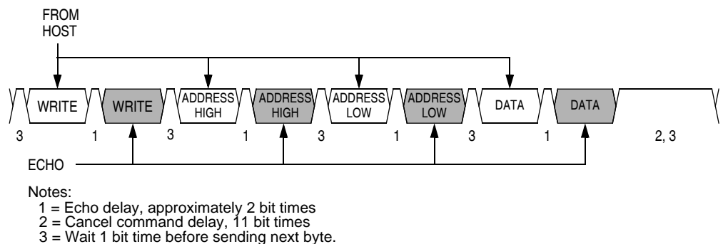
Figure 17-11. Write Transaction
