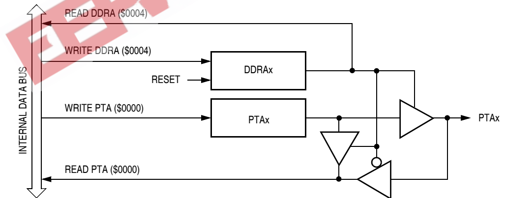
Figure 12-4. Port A I/O Circuit
