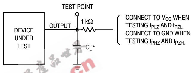
Figure 7. Test Circuit
