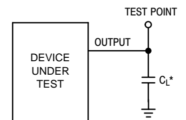
Figure 6. Test Circuit
