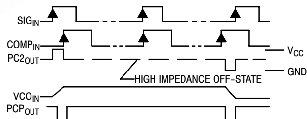
Figure 9. Typical Waveforms for PLL Using Phase Comparator 2
