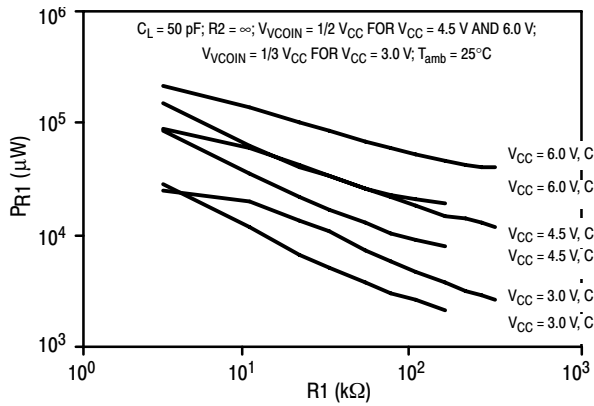
Figure 16. Power Dissipation versus R1
