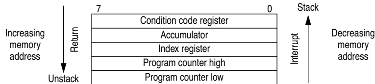
Figure 9-2 Stacking order
