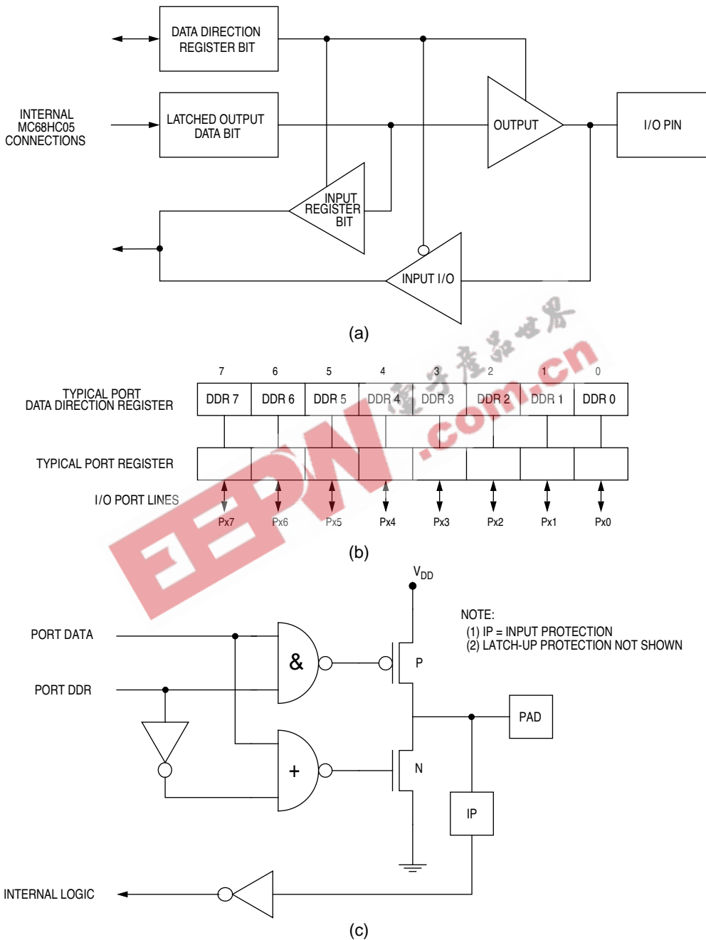
Figure 2-3 Parallel Port I/O Circuitry
