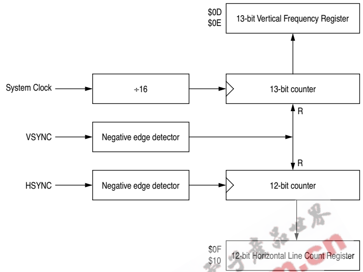
Figure 8-4 Sync Signal Counters Block Diagram
