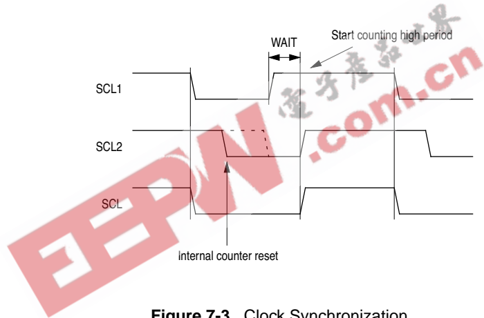
Figure 7-3 Clock Synchronization
