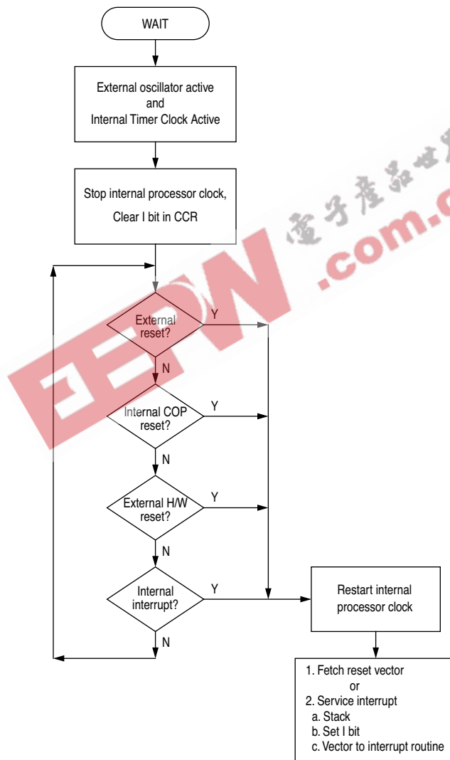
Figure 10-1 WAIT Flowchart
