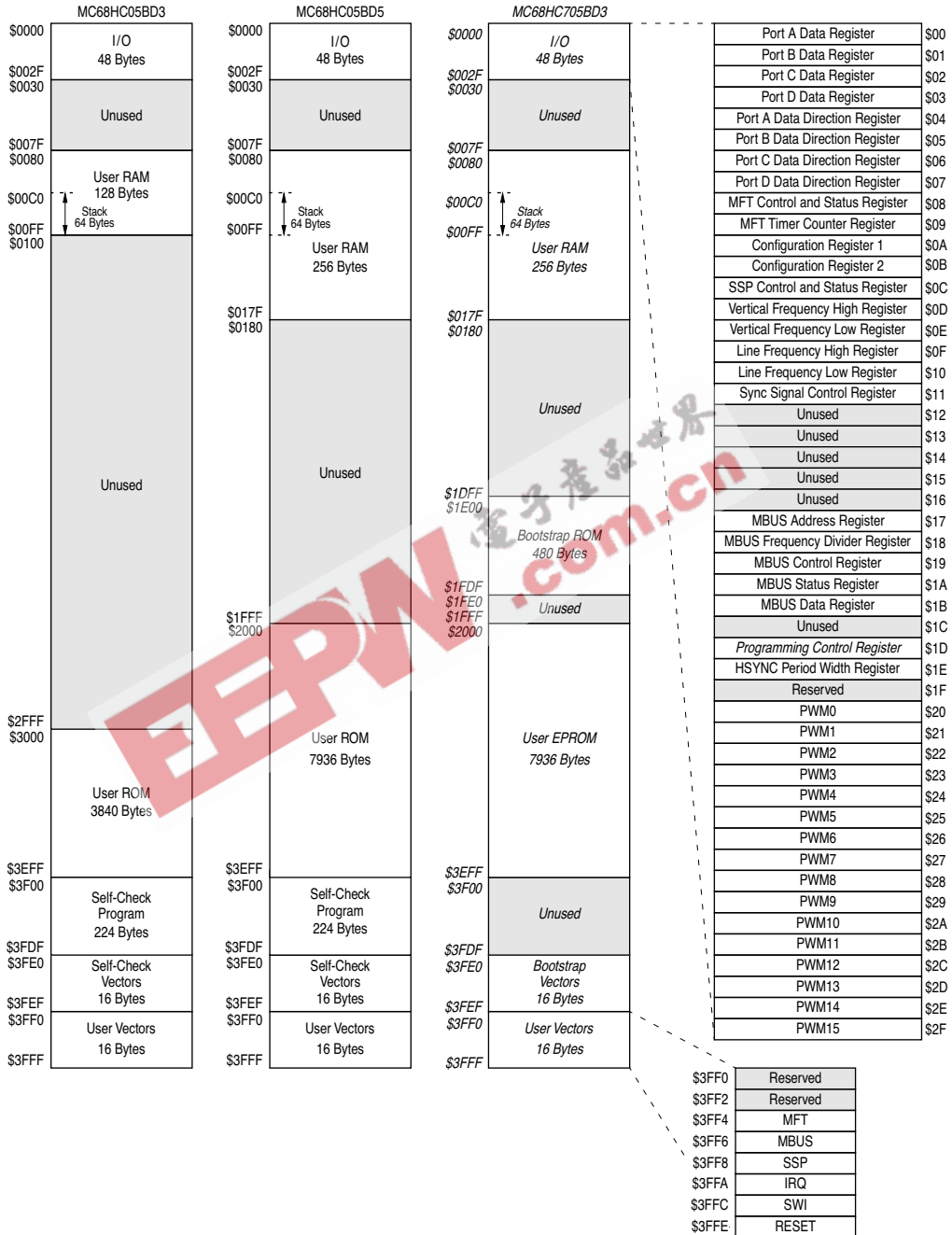
Figure 3-1 Memory Map
