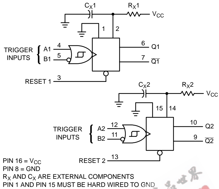
Figure 2. Logic Diagram
