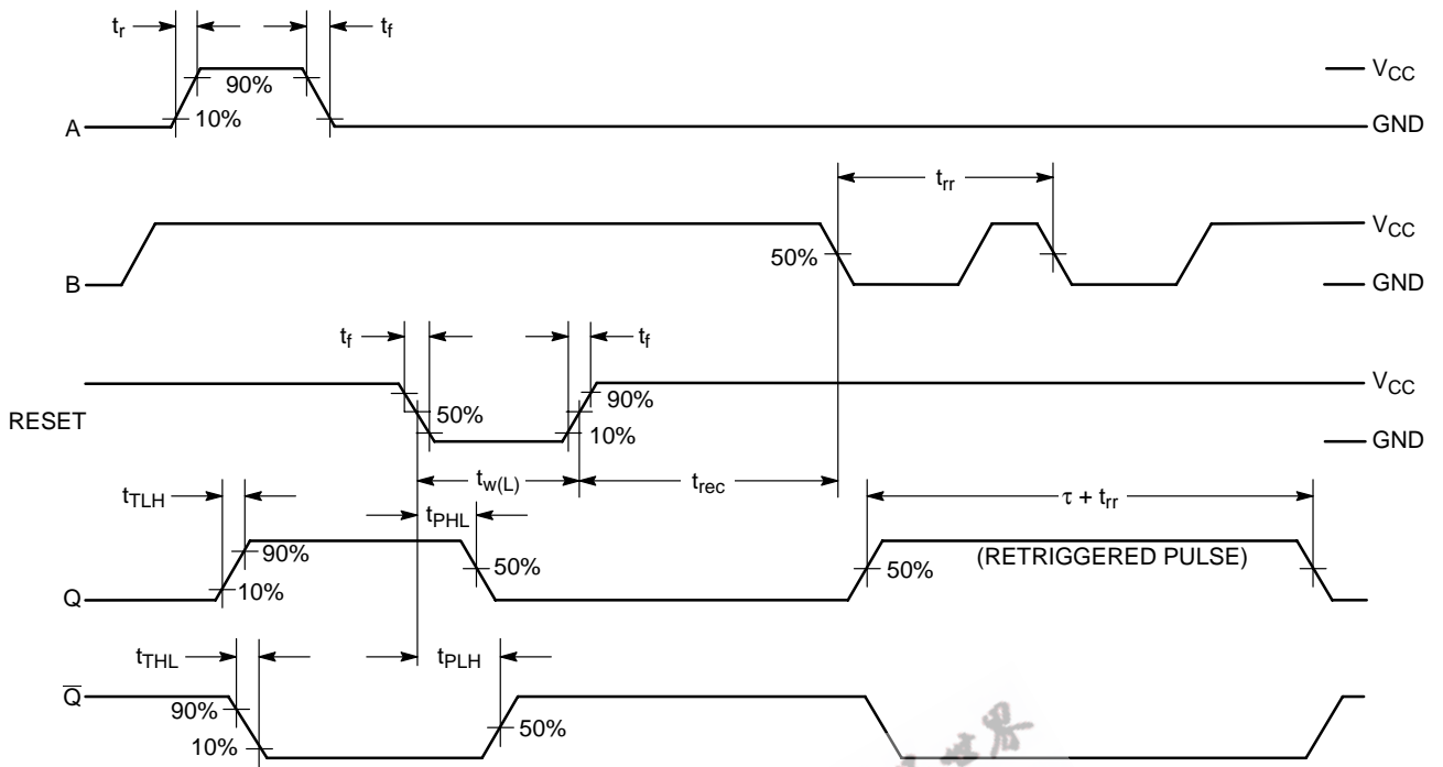
Figure 9. Switching Waveform
