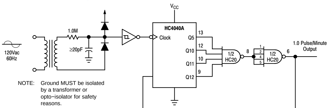
Figure 9. Time-Base Generator
