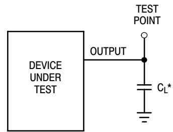
Figure 6. Test Circuit
