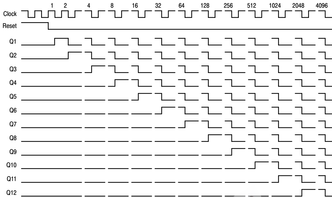
Figure 8. Timing Diagram
