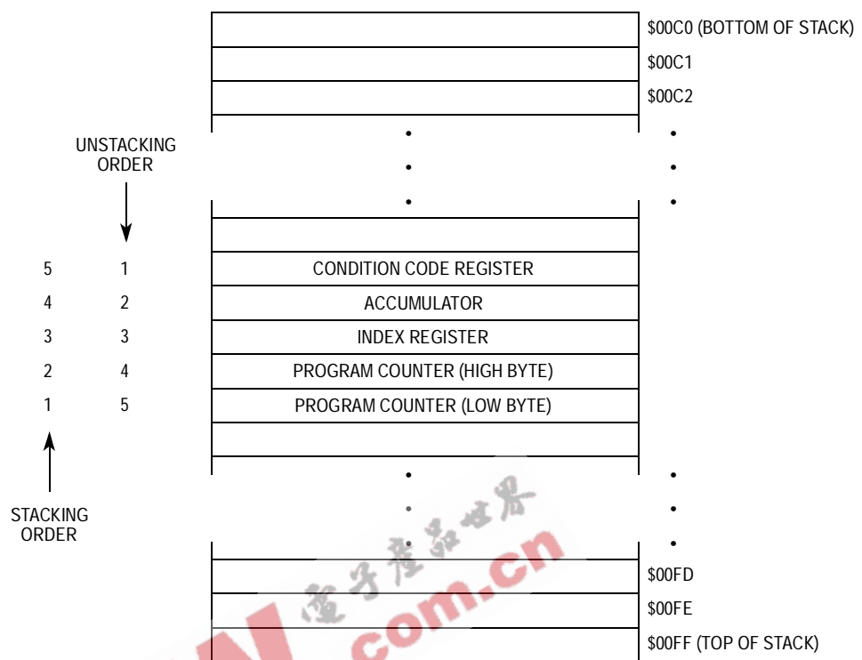
Figure 4-3. Stacking Order
