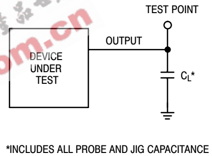
Figure 5. Test Circuit
