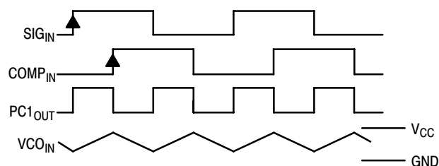
Figure 8. Typical Waveforms for PLL Using Phase Comparator 1
