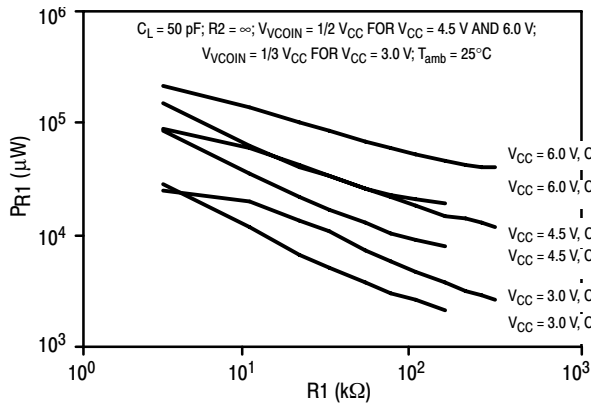
Figure 16. Power Dissipation versus R1
