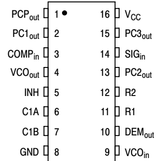
Figure 1. Pin Assignment
