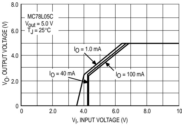
Figure 1. Dropout Characteristics
