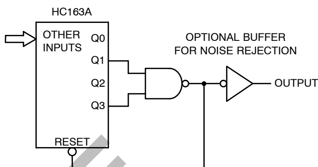
Figure 17. Modulo-11 Counter
