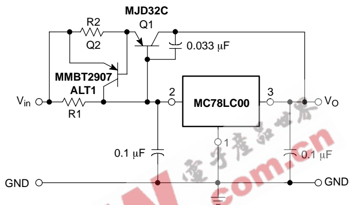
Figure 23. Current Boost Circuit with Overcurrent Limit Circuit
