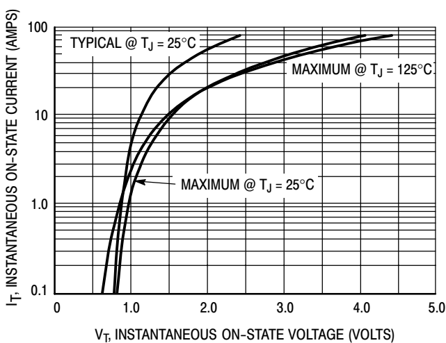
Figure 3. On-State Characteristics
