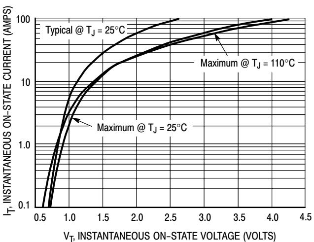
Figure 3. On-State Characteristics
