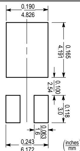
Figure 1. Minimum Pad Sizes for Surface Mounting
