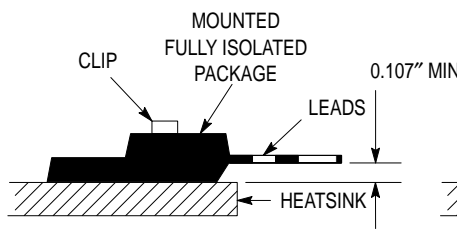
Figure 23. Clip Mounting Position for Isolation Test Number 2
