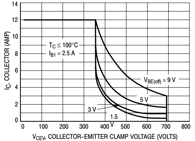
Figure 2. Reverse Bias Switching Safe Operating Area
