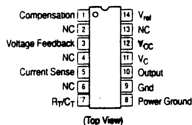
PIN CONNECTIONS
