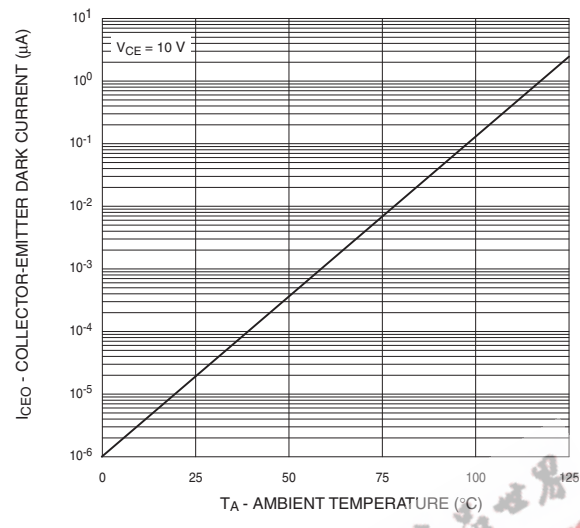
Fig. 19 Dark Current vs. Ambient Temperature (Black Package)
