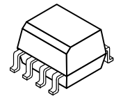
CASE 846-01, STYLE 3 PLASTIC
