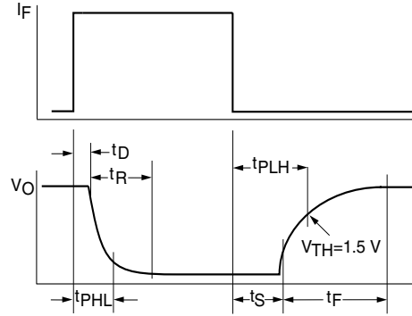
Figure 6. Switching Waveform
