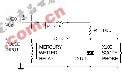
Static dv/dt Test Circuit
