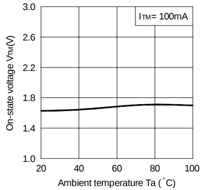
Fig.5 On-state Voltage vs. Ambient Temperature
