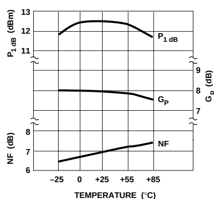
Figure 3. Output Power at 1 dB Gain Compression, NF and Power Gain vs. Case Temperature, f = 1.0\ \text{GHz} , I_d = 50\ \text{mA} .
