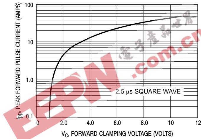
Figure 7. Clamping Voltage versus Peak Pulse Current (Forward Direction)
