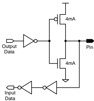
CMOS Pin (Output Mode) Pxoe = 1
