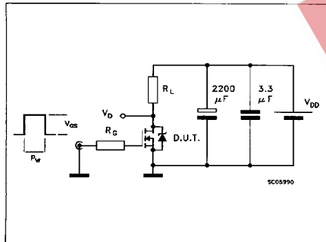
Fig. 3: Switching Times Test Circuits For Resistive Load
