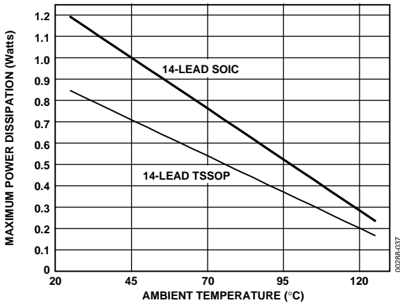
Figure 37. Maximum Power Dissipation vs. Temperature for 14-Lead Package Types
