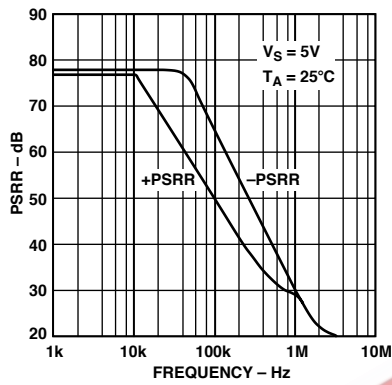
Figure 22. PSRR vs. Frequency
