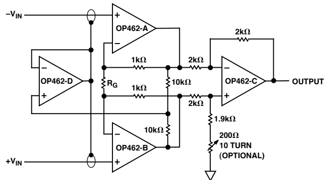
Figure 41. A High Speed Instrumentation Amplifier
