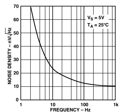
Figure 18. Voltage Noise Density vs. Frequency
