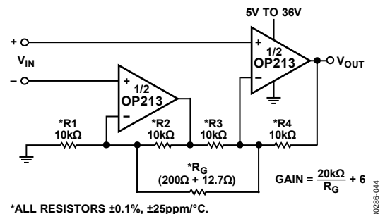
Figure 45. Ultralow Noise, Single Supply Instrumentation Amplifier
