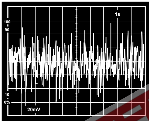
Figure 36. Input Voltage Noise @ \pm 15\text{ V} (20 nV/div)
