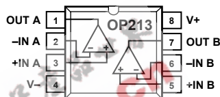
Figure 3. 8-Lead PDIP
