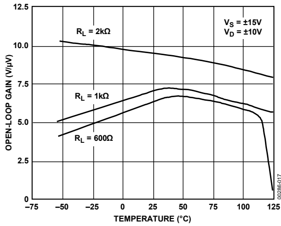
Figure 17. OP413 Open-Loop Gain vs. Temperature
