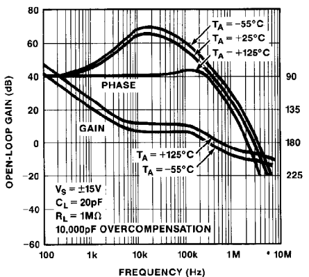
OPEN-LOOP GAIN, PHASE vs FREQUENCY ( C_{OC} = 10,000pF )
