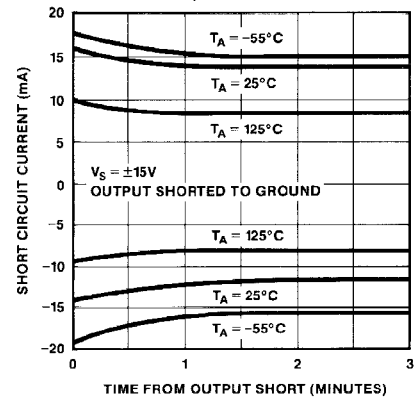
SHORT CIRCUIT CURRENT vs TIME, TEMPERATURE
