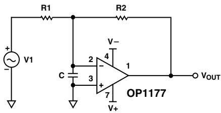
Figure 11. EMI Reduction
