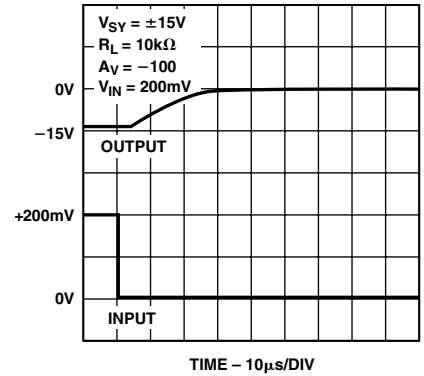
TPC 12. Positive Overtolerance Recovery
