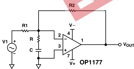
Figure 12. Compensation Using Input RC Network
