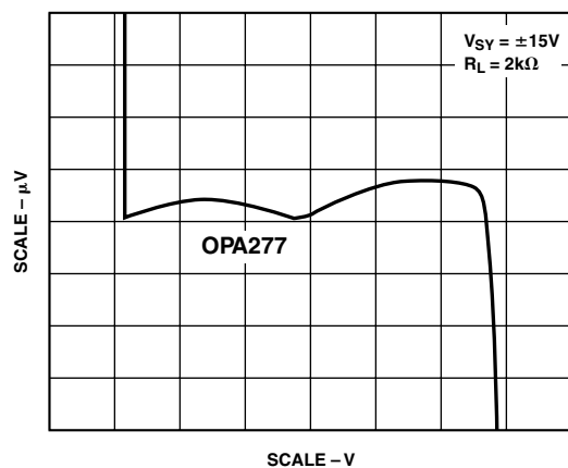
Figure 2. Gain Linearity
