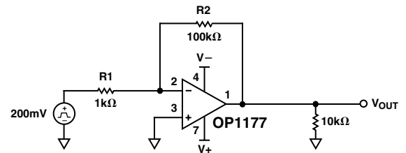
Figure 4. Test Circuit for Overload Recovery Time
