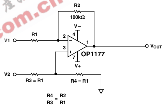
Figure 13. Difference Amplifier
