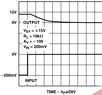
TPC 13. Negative Overtolerance Recovery
