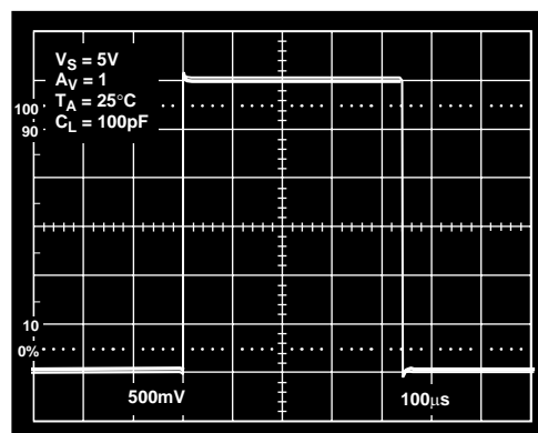
Figure 32. Large Signal Transient Response
