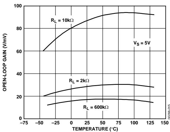
Figure 15. OP462 Open-Loop Gain vs. Temperature
