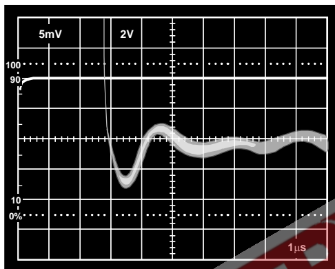
Figure 49. Negative Slope Settling Time
