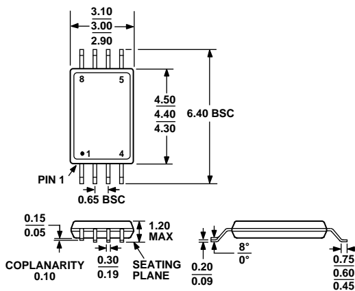
Figure 53. 8-Lead Thin Shrink Small Outline Package [TSSOP] (RU-8) Dimensions shown in millimeters
