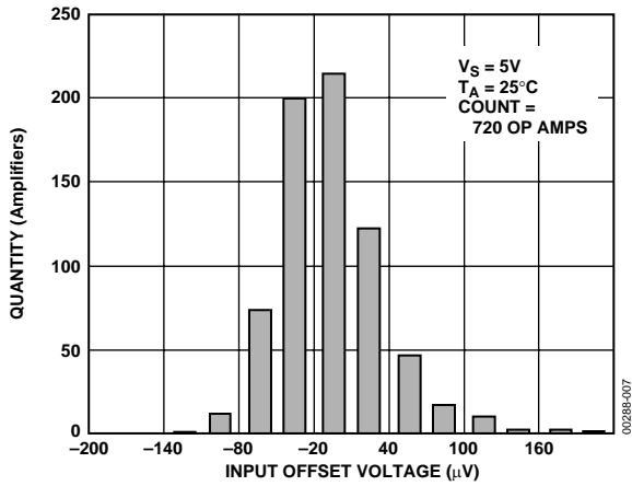
Figure 7. OP462 Input Offset Voltage Distribution
