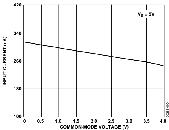
Figure 9. OP462 Input Bias Current vs. Common-Mode Voltage
