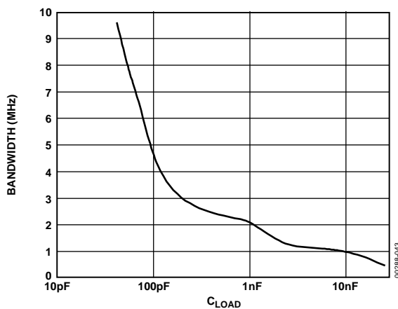
Figure 43. Unity-Gain Bandwidth vs. C_{LOAD}
